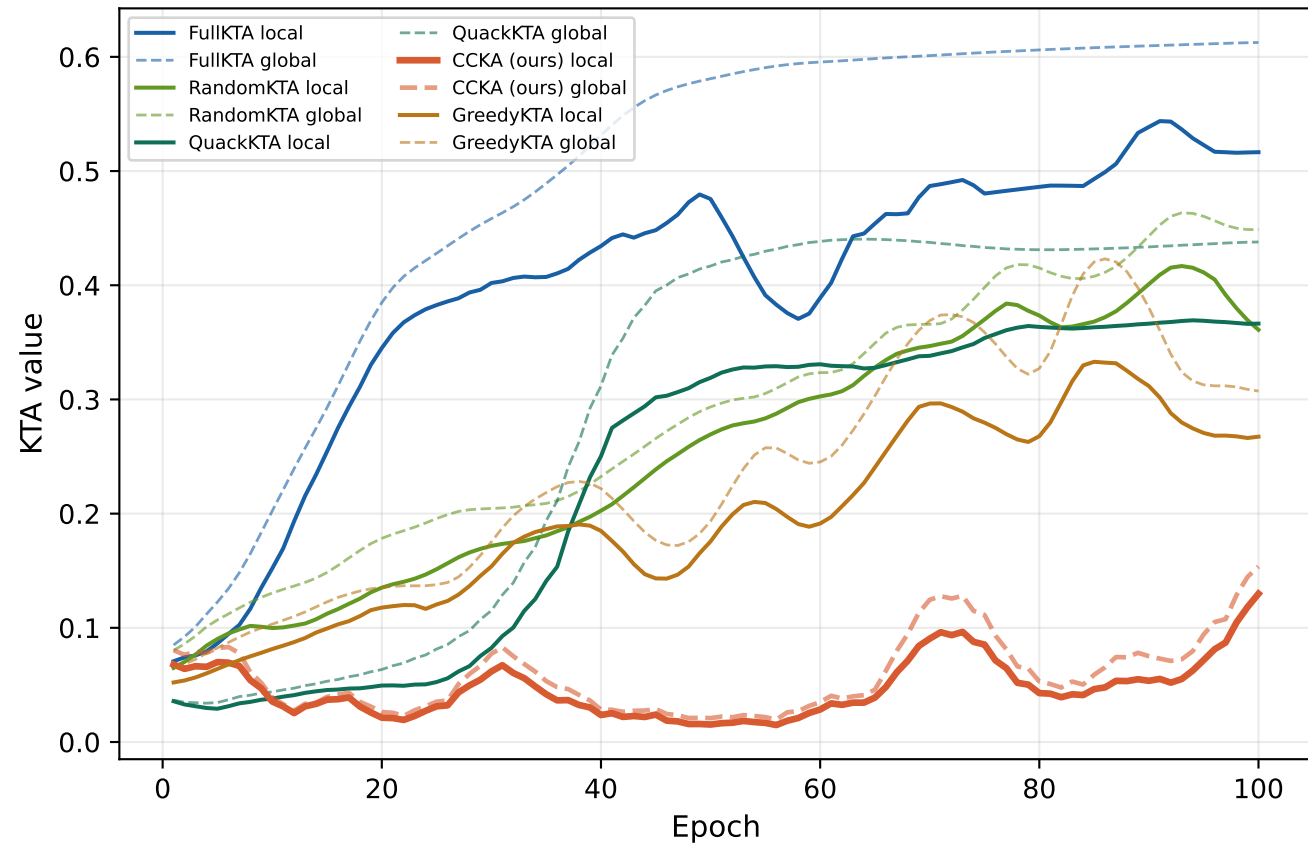
Local SV-KTA (solid) vs Global KTA (dashed)
