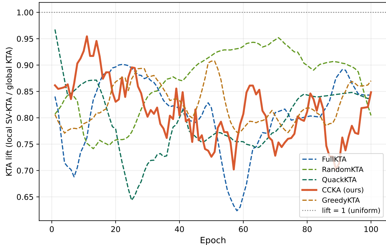
SV-3: KTA lift at support vectors — checkerboard
