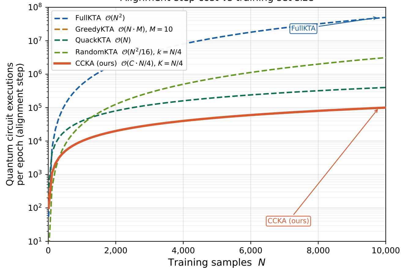
Alignment-step cost vs training set size
