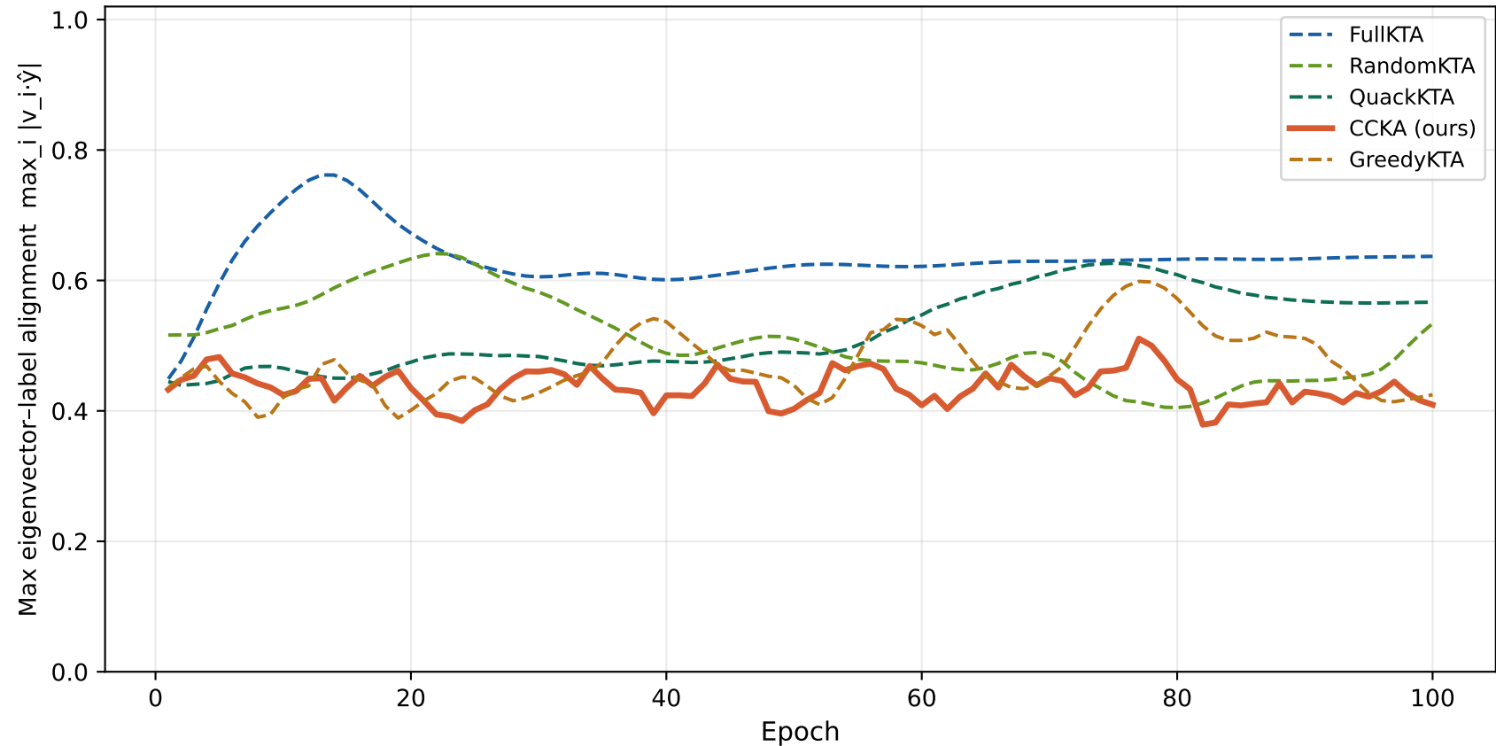
Best-aligned eigenvector over training — corners CCKA collapse ( \sim ep64) should show a sharp drop here
