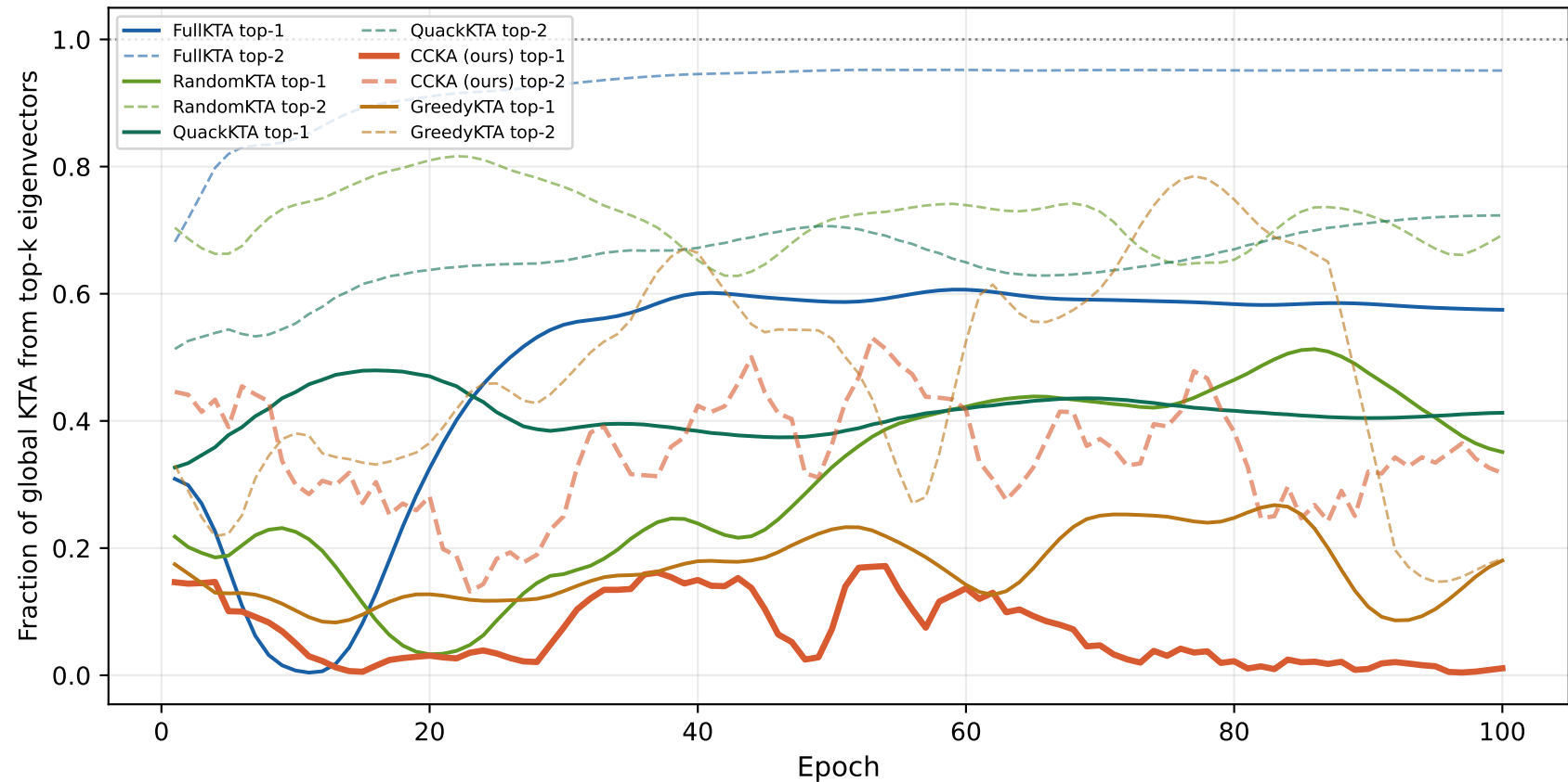
KTA decomposition by rank — corners Near 1.0 = essentially all KTA in the top 1-2 directions (low-rank)
