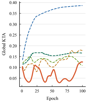
(b) Global KTA
