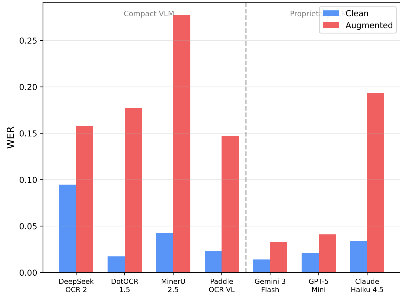
Word Error Rate (WER)
