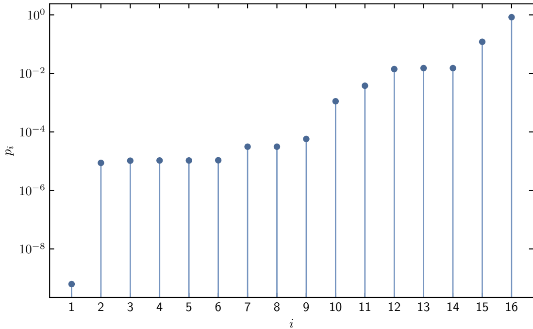
Spectrum of \rho
