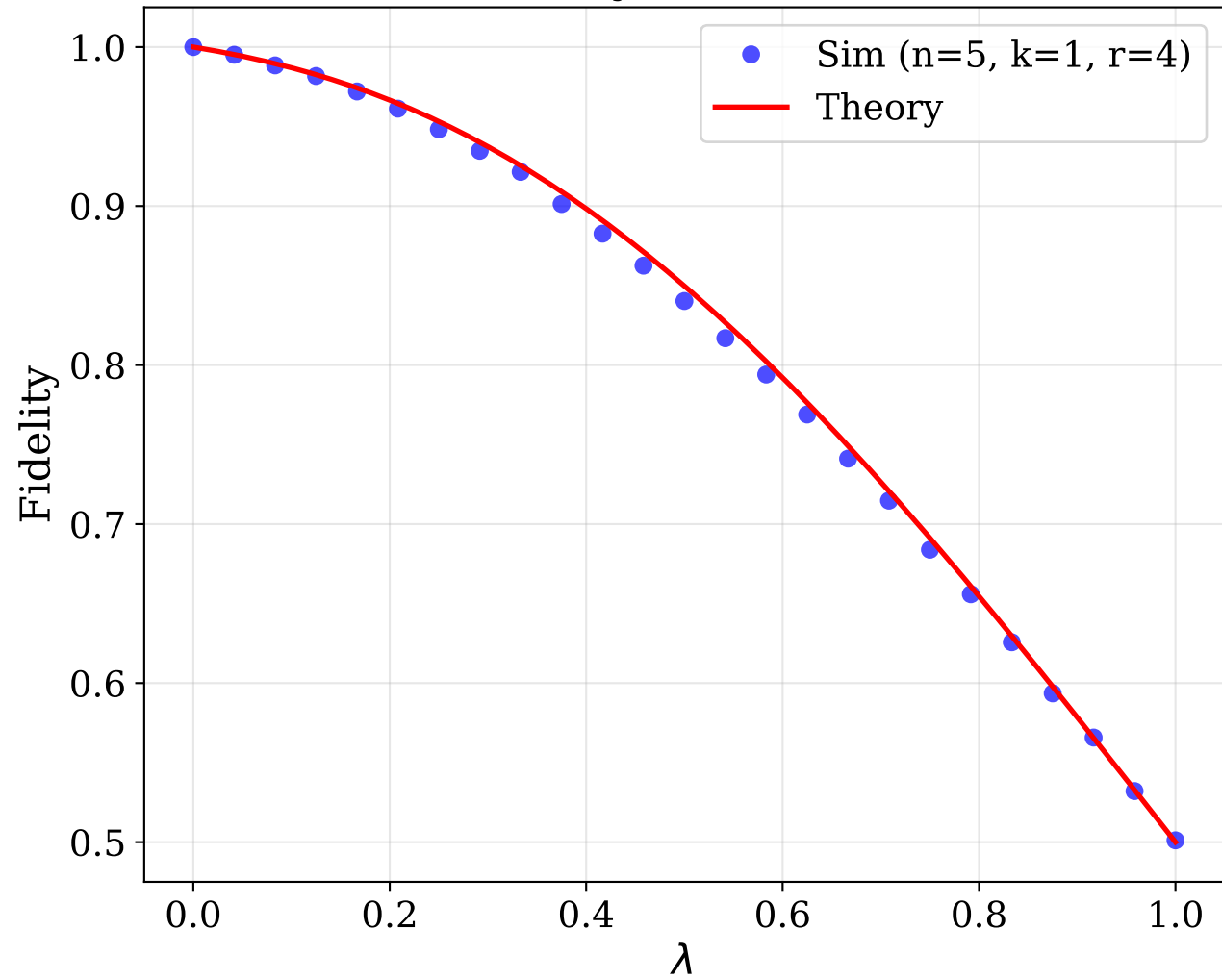
Fidelity vs. \lambda (n=5)
