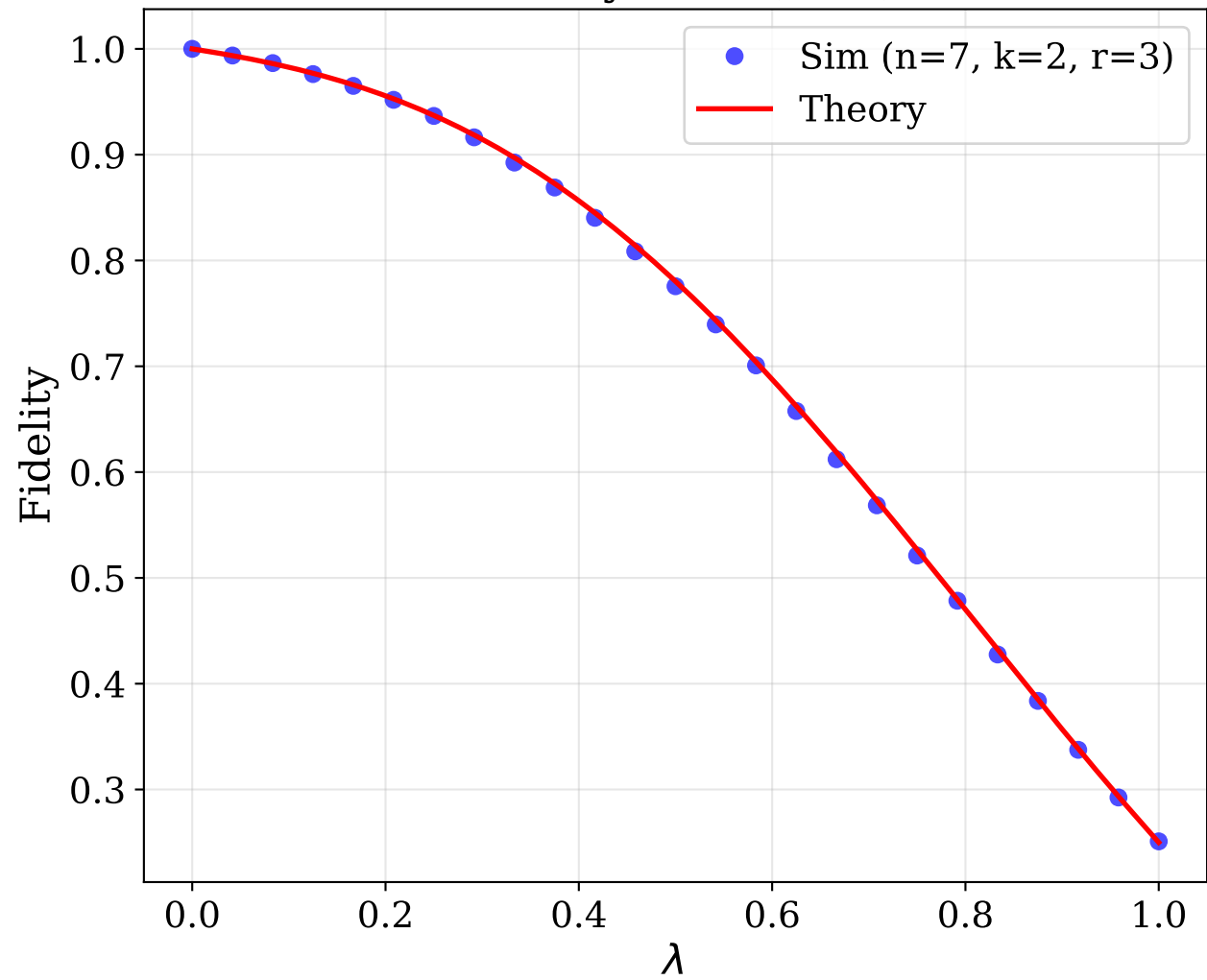
Fidelity vs. \lambda (n=7)
