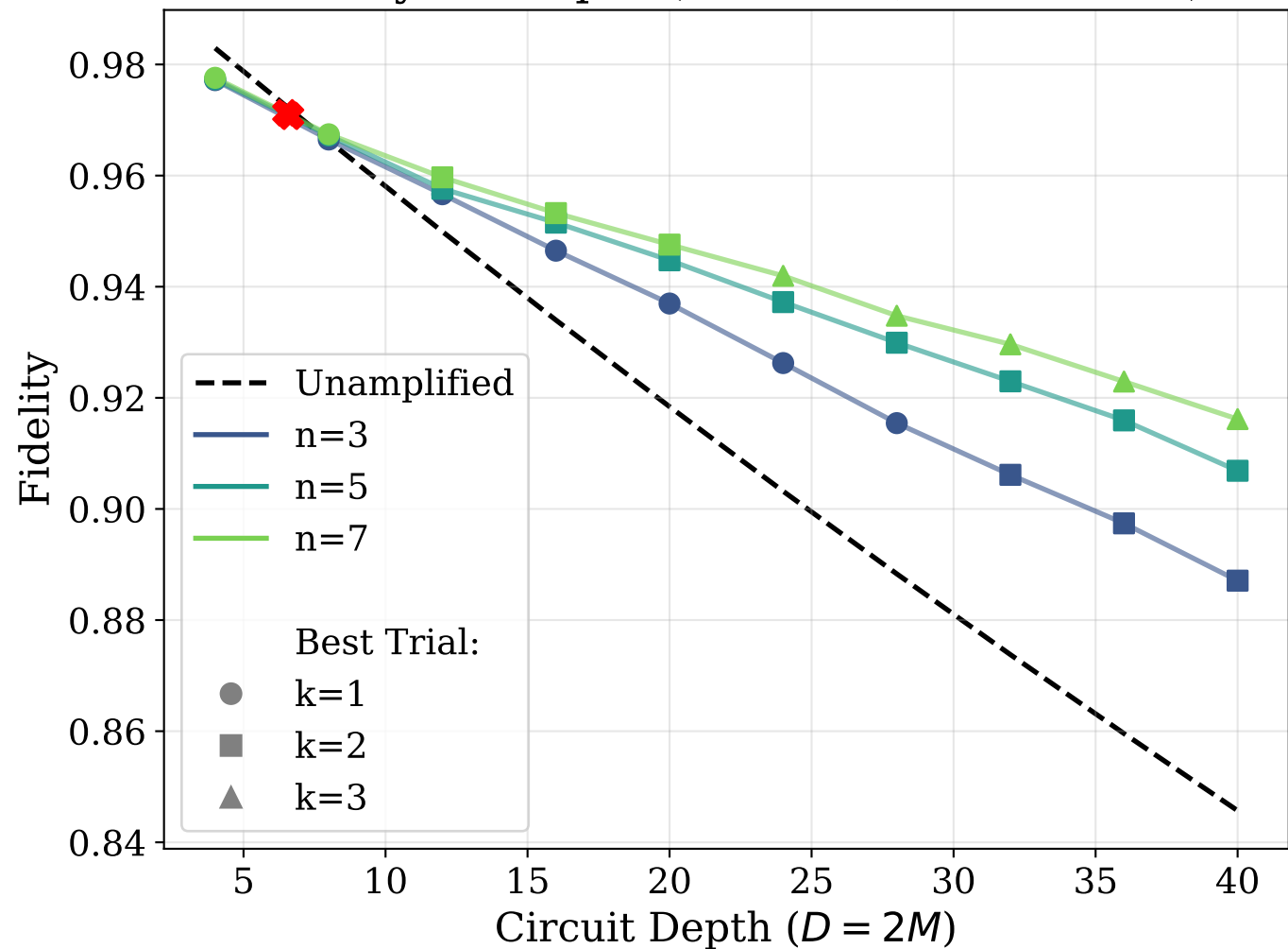
Fidelity vs. Depth ( \epsilon = 0.001 , Trials=max)
