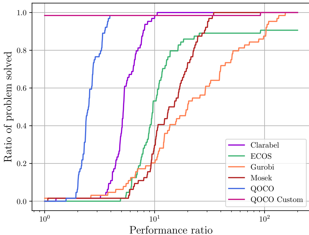
Performance Ratio
