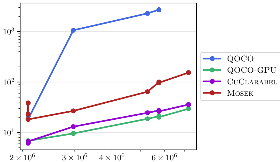
Tv Denoising
