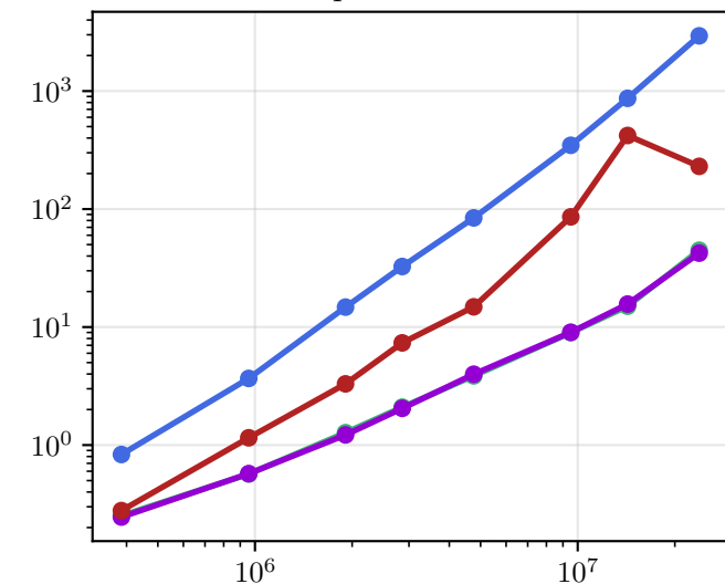
Tv Denoising
