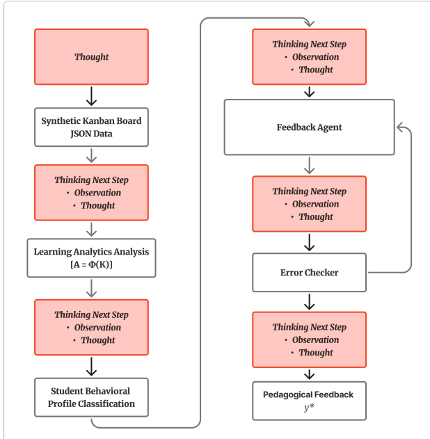
Fig. 2: ReAct agent mechanism structure.
