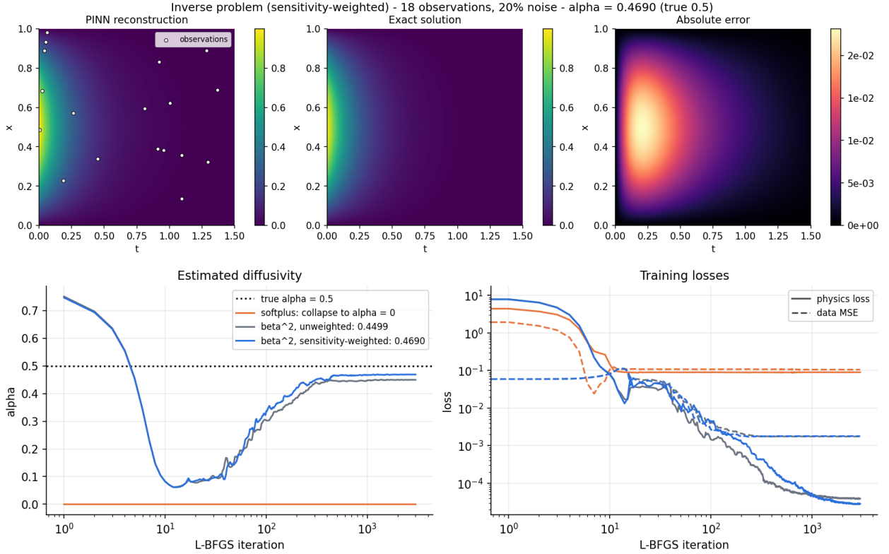
Figure 2: Top: sensitivity-weighted inverse reconstruction. Bottom: \alpha and loss histories of the three variants (python scripts/inverse.py).
