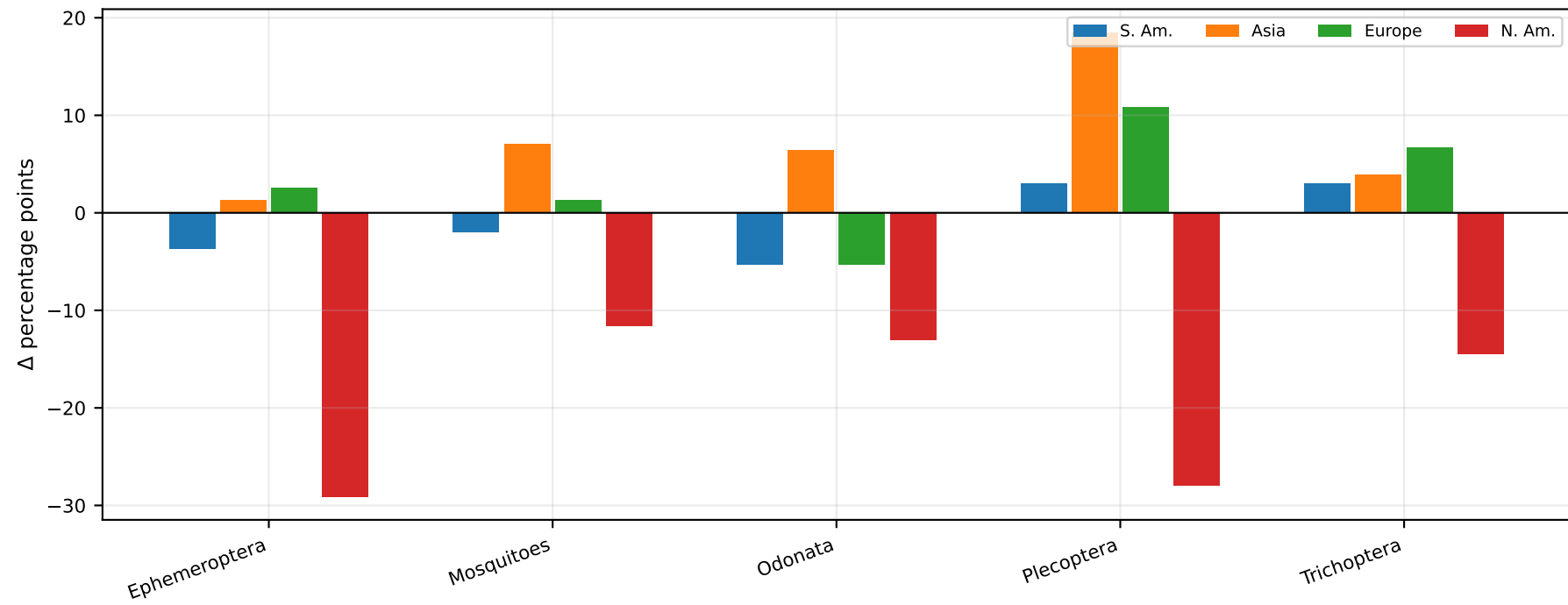
RQ2 — Continental shift (mean 2023–2025 – mean 2010–2012)
