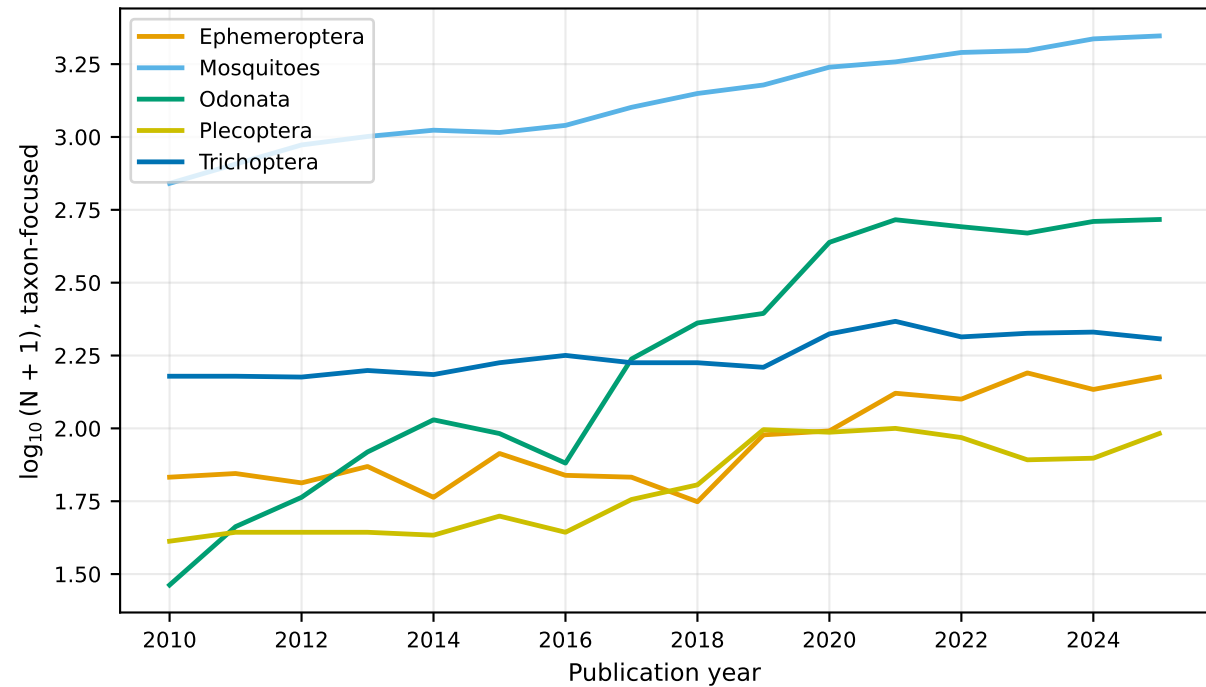
Cross-taxon publication volume (log scale, comparable shape)
