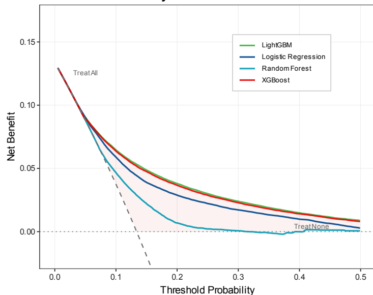
d Decision Curve Analysis
