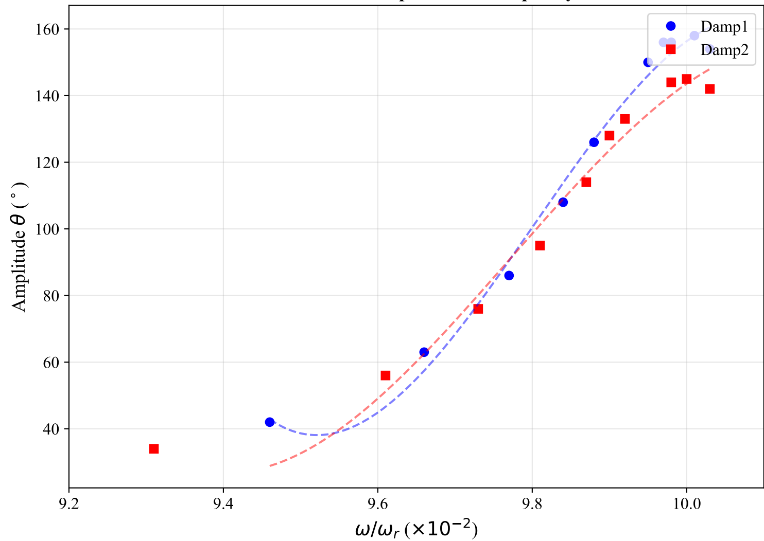
Resonance Curves: Amplitude vs. Frequency Ratio
