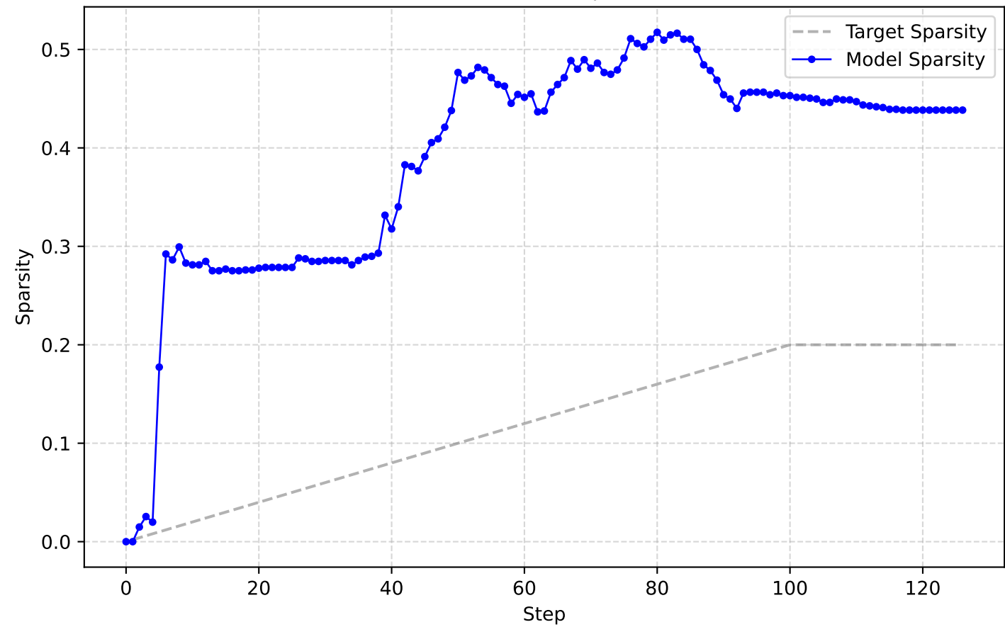
Task: Summarization
