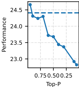
Summarization
