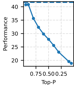
Single-QA
