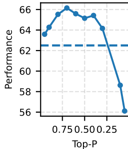
Few-Shot
