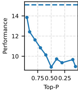
Code
