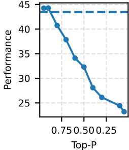
Multi-QA
