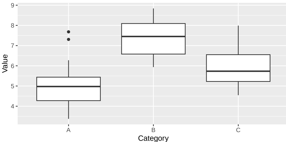
Figure 7: Boxplot example
