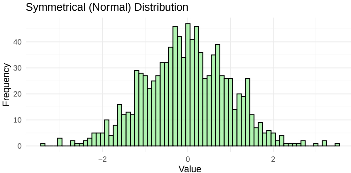
Figure 8: Symmetrical histogram
