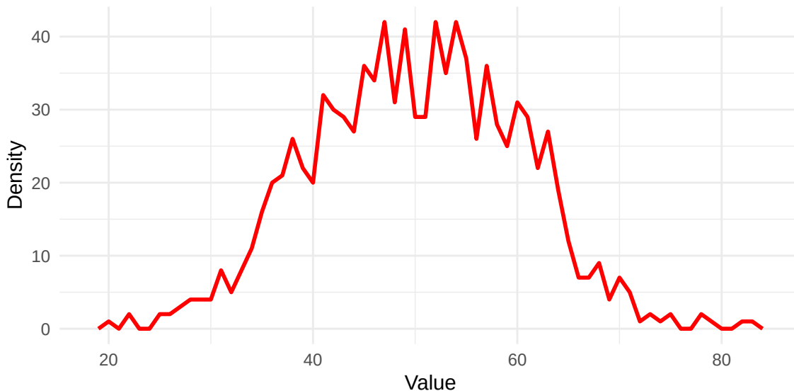
Figure 6: Frequency polygon
