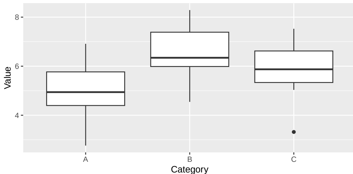
Figure 7: Boxplot example
