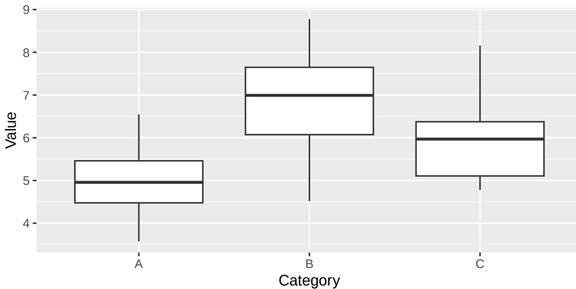
Figure 6: Boxplot example
