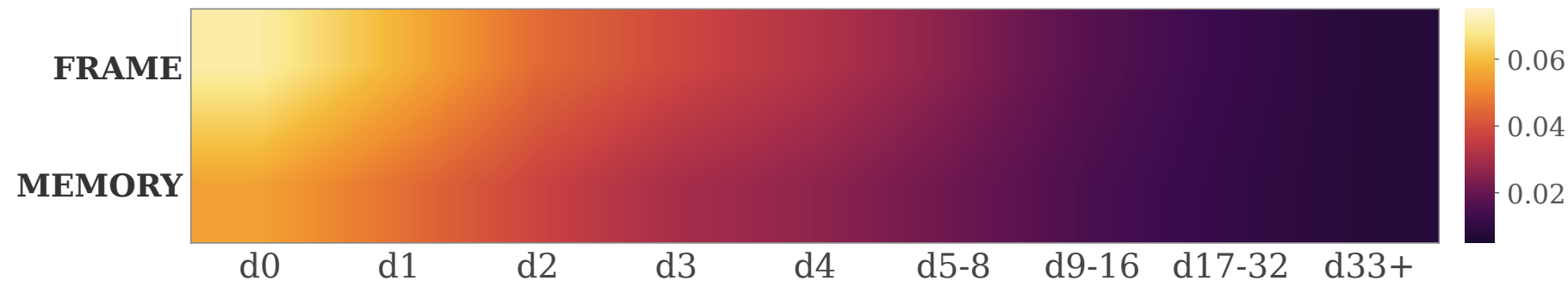
(b) Stage3: Answer Attention Distribution
