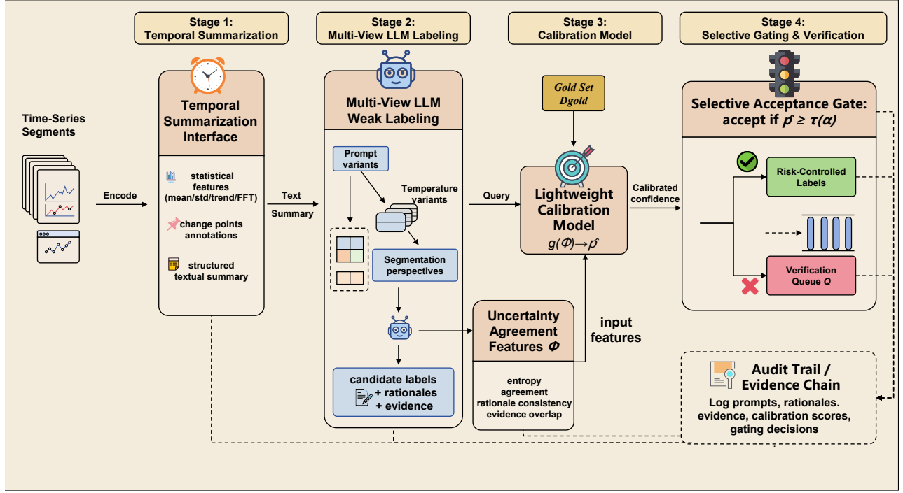
Figure 1: CALM-TS converts time-series segments into structured textual summaries (Stage 1), queries an LLM with diverse prompts, temperatures, and context windows to elicit multi-view labels with rationales (Stage 2), learns a lightweight calibrator over disagreement features on a small gold set (Stage 3), and selectively gates accepted labels under a finite-sample risk budget while routing uncertain instances to cost-aware verification (Stage 4). The audit trail from each accepted label back to the LLM’s reasoning and calibration score is preserved end-to-end.
