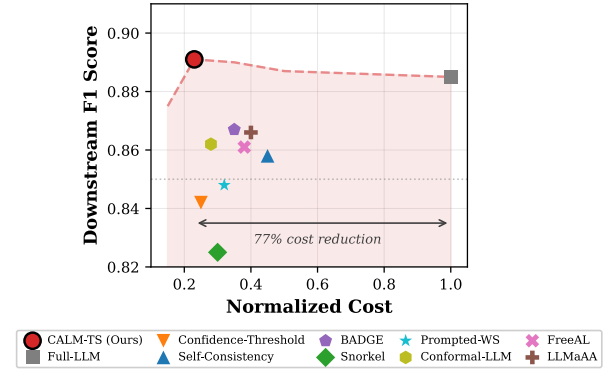
Figure 2: Cost-performance trade-off on MIMIC-III with the GPT-4 backbone. Takeaway. CALM-TS Pareto-dominates Full-LLM, Self-Consistency, Confidence-Threshold, Snorkel, and BADGE on F1 versus normalized cost. Per-seed \alpha -compliance for every method is reported in Table 1 and the paired sign-test analysis of Section 5; the corresponding PhysioNet operating point is read directly from Table 1.
