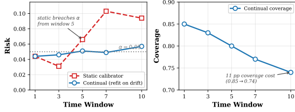
Figure 3: Per-window risk under streaming drift on Yahoo S5. The static calibrator drifts above \alpha = 0.05 from window 5 onward; the continual variant refits on detector triggers and holds mean risk at 0.049 at an 11-point coverage cost.
