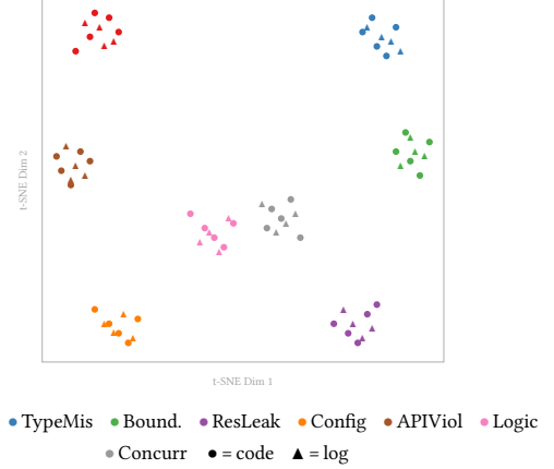
Figure 4: Schematic of the fault-type layout in the aligned embedding space. This panel is illustrative, not a rendering of measured coordinates: it shows one representative subsample per type for readability, and the full 25,982-point t-SNE is provided in the replication package. The one measured quantity reported here is the 72% cross-modal nearest-neighbour overlap rate on the full sample; all quantitative claims about the embedding space rest on that number rather than on this drawing.
