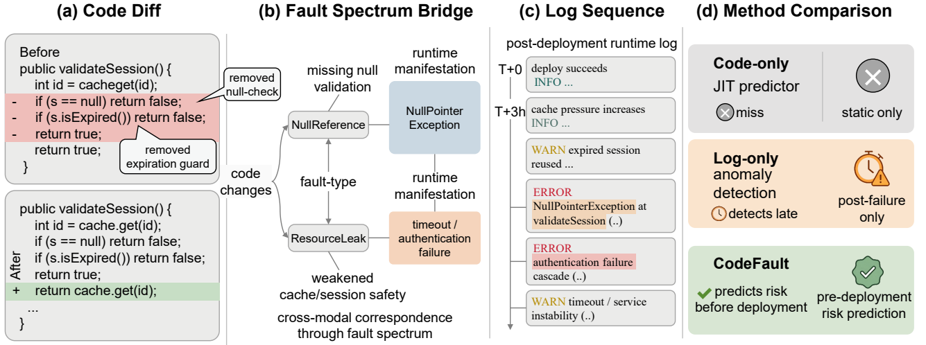
Figure 1: Motivating example: a removed null-check in validateSession() triggers cascading NullPointerException errors post-deployment. Code-only methods miss the runtime-dependent fault; log-only methods detect it only after failure cascades. CODEFAULT bridges both modalities via the fault spectrum, predicting the risk before deployment.
