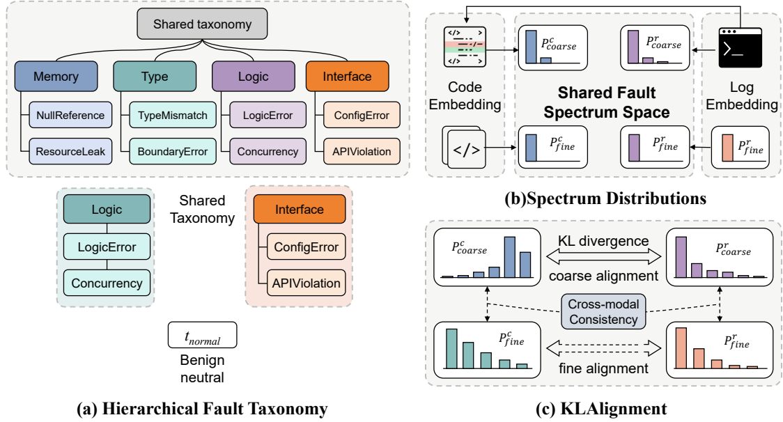
Figure 2: Hierarchical fault taxonomy ( K_c=4 coarse categories on the left, K_f=8 fine categories on the right, plus the benign type t_{\text{normal}} ). Code and log modalities are independently projected into this shared space via softmax heads P_c and P_r at each granularity; KL-divergence alignment enforces cross-modal consistency level by level. The dashed arrows show the marginalization map \text{Margin}(\cdot) used by the hierarchical consistency constraint in §3.5.
