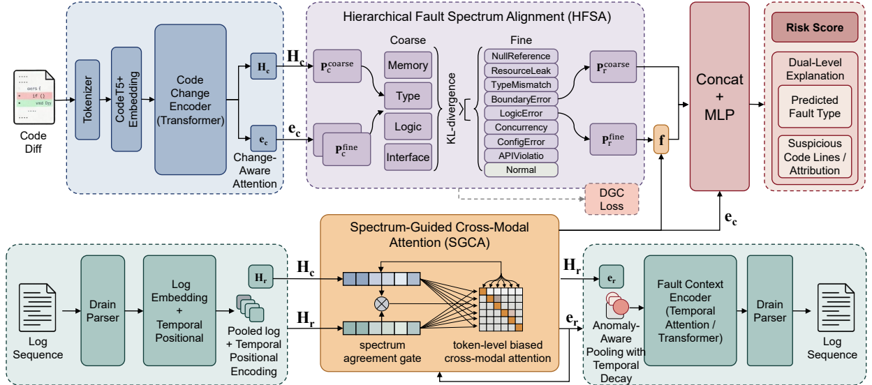
Figure 3: Architecture of CODEFAULT. Code and log modalities are encoded, projected into a hierarchical fault spectrum space (HFSA), and fused via token-level spectrum-guided cross-modal attention (SGCA).
