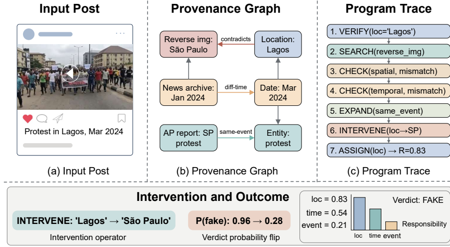
Figure 3: Qualitative case study: a recontextualized protest video. (a) Input post with fabricated caption. (b) Provenance graph connecting claim slots to retrieved evidence via typed edges (contradicts, diff-time, same-event). (c) 7-step verification program trace. (d) The INTERVENE operator replaces “Lagos” with evidence-supported “São Paulo,” flipping verdict probability from 0.96 to 0.28 and assigning primary responsibility R=0.83 to the location fabrication.
