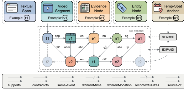
Figure 4: Schema of the temporal-multimodal provenance graph. Five node types (top) are connected via seven typed edges (bottom). The graph is dynamically expanded by the verification program’s SEARCH and EXPAND operators. Avg: 22.3 \pm 8.1 nodes, 58.2 \pm 21.4 edges.
