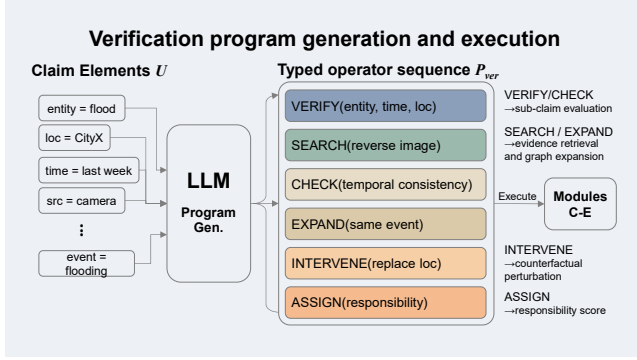
Figure 2: Verification program generation and execution. The LLM generates a typed operator sequence P_{\text{ver}} from parsed claim elements. Each operator has well-defined semantics: VERIFY/CHECK trigger sub-claim evaluation, SEARCH/EXPAND drive evidence retrieval and graph expansion, INTERVENE plans counterfactual perturbations, and ASSIGN computes responsibility scores.
