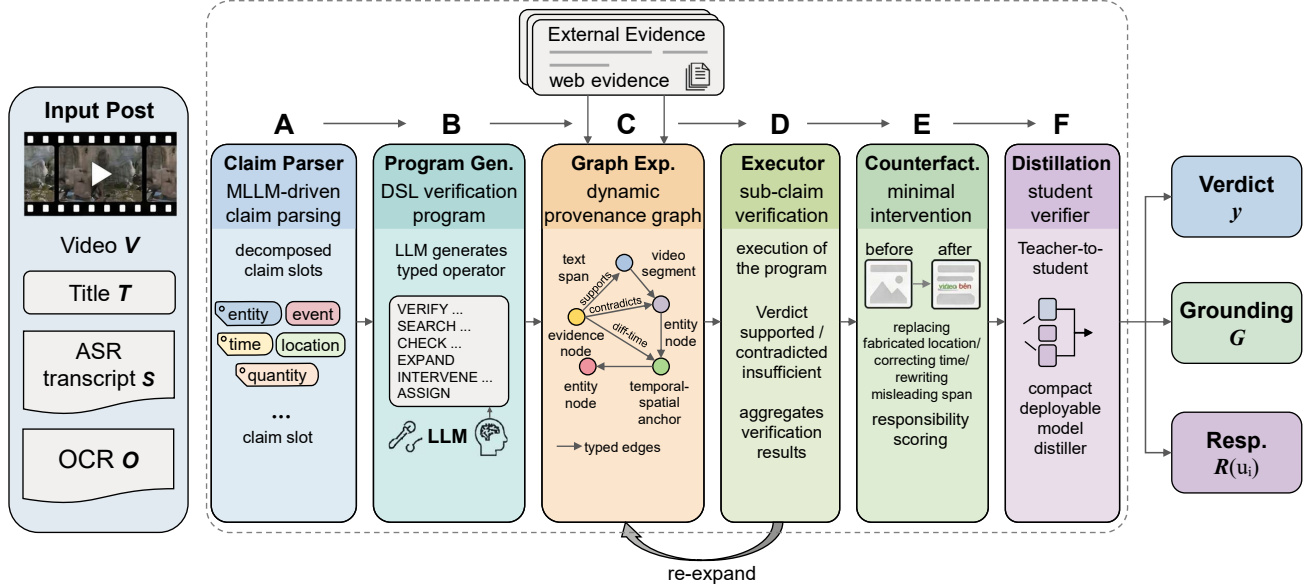
Figure 1: Overview of PROG-TRACE. An LLM-driven verification framework that parses multimodal claims into structured slots (Module A), generates an executable verification program (Module B), uses it to orchestrate evidence retrieval and dynamic provenance graph expansion (Module C), executes sub-claim verification with verdict aggregation (Module D), performs LLM-planned minimal counterfactual interventions for responsibility attribution (Module E), and distills the full reasoning trace into a compact student verifier (Module F).
