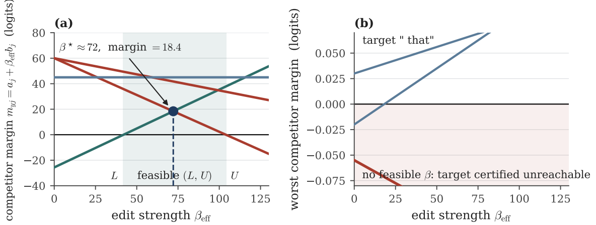
Figure 4: The certificate is one-dimensional linear feasibility (Proposition 1, Corollary 1). Each line is a competitor margin m_{yj}(\beta_{\text{eff}}) = a_j + \beta_{\text{eff}}b_j ; the target wins where all lie above zero. (a) A reachable target: the feasible interval (L, U) is non-empty and \beta^* maximizes the worst-case margin (values from betastar.json ). (b) An unreachable target (“that”, blocked by “,”): a competitor with a_j \leq 0 , b_j \leq 0 stays below zero for every \beta_{\text{eff}} , so the certificate refuses it before injection. Representative competitor lines drawn to scale around the measured operating point.
