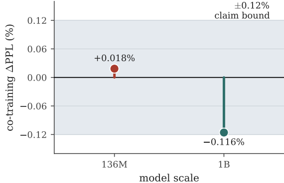
Figure 8: Signed co-training perplexity delta, (\text{hybrid} - \text{baseline})/\text{baseline} , per scale: +0.018% at 136M (co-training marginally worse) and -0.116\% at 1B (co-training better). The shaded band is the paper’s \pm 0.12\% no-tax claim bound; both scales fall inside it. Data: g2a_no_tax.json , g3a_no_tax.json , notax_params.json .
