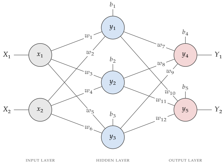
Figure 3.2 The network in Exercise 3.2: two inputs, three hidden nodes and two output nodes.
