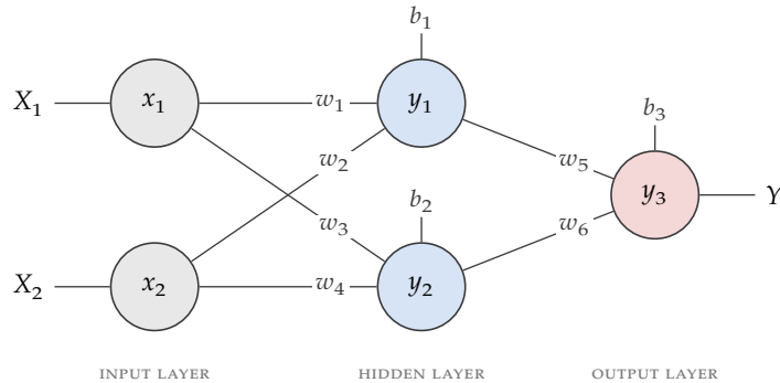
Figure 3.1 The network in Exercises 3.1 and 3.3: two inputs, two hidden nodes and one output node.
