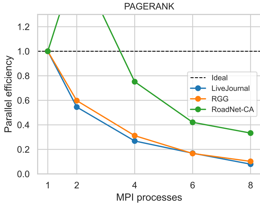
Parallel Efficiency vs. Number of MPI Processes
