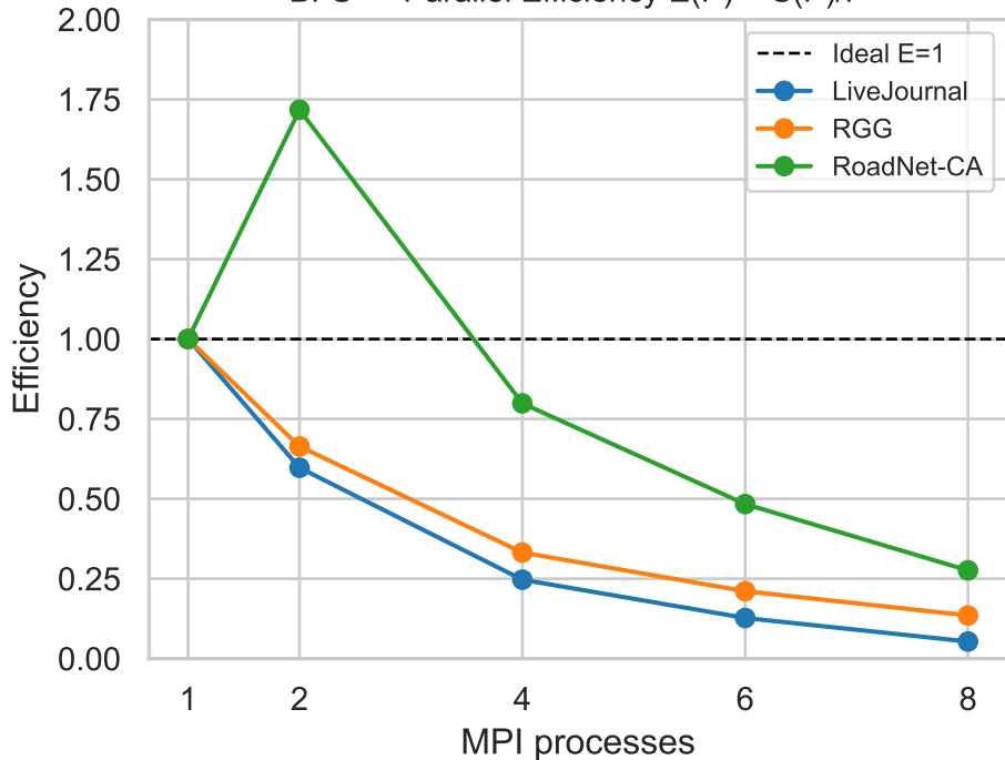
BFS — Parallel Efficiency E(P) = S(P)/P
