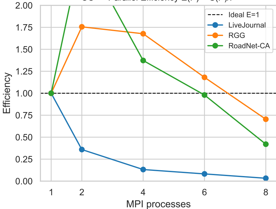
CC — Parallel Efficiency E(P) = S(P)/P
