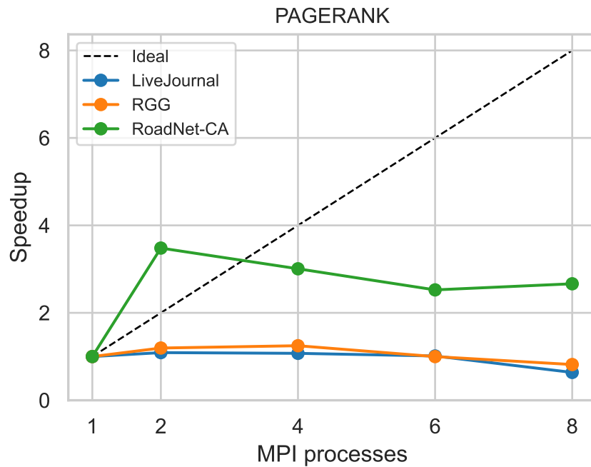
Speedup vs. Number of MPI Processes
