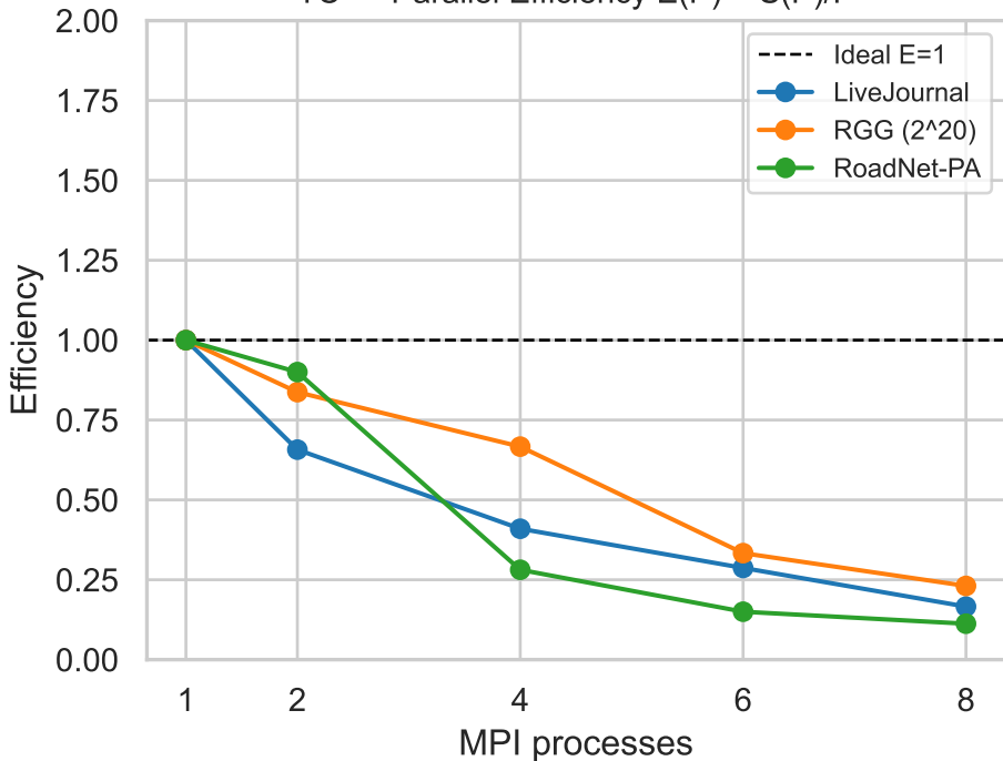
TC — Parallel Efficiency E(P) = S(P)/P
