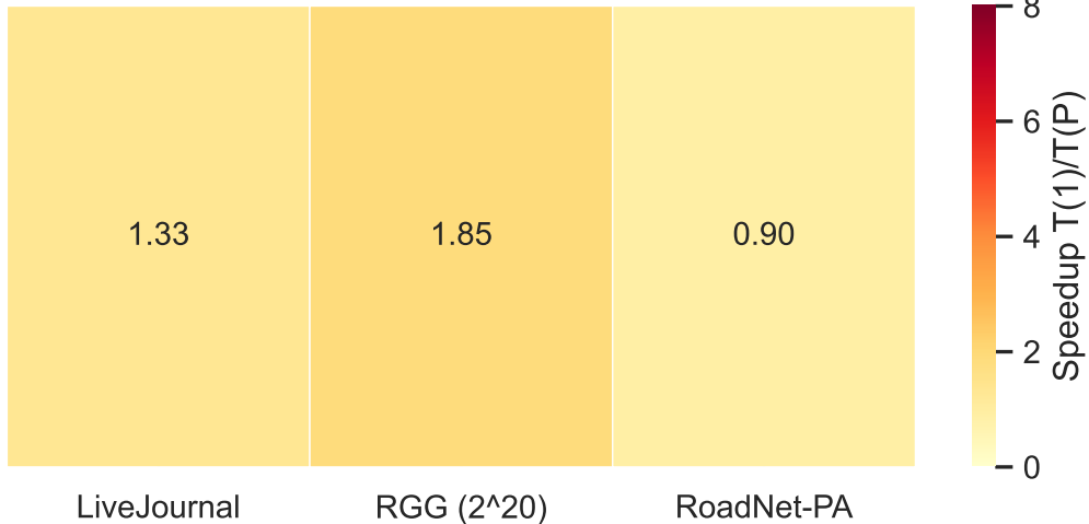
Speedup T(1)/T(P) at 8 MPI processes (ideal = 8)
