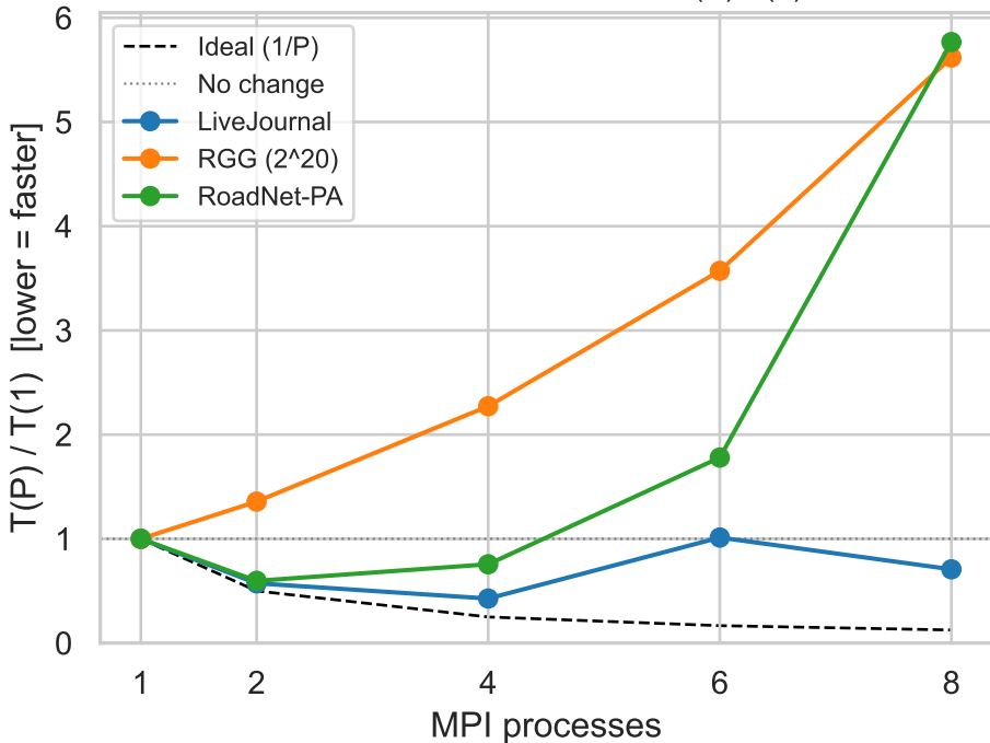
SSSP — Normalized Time T(P)/T(1)
