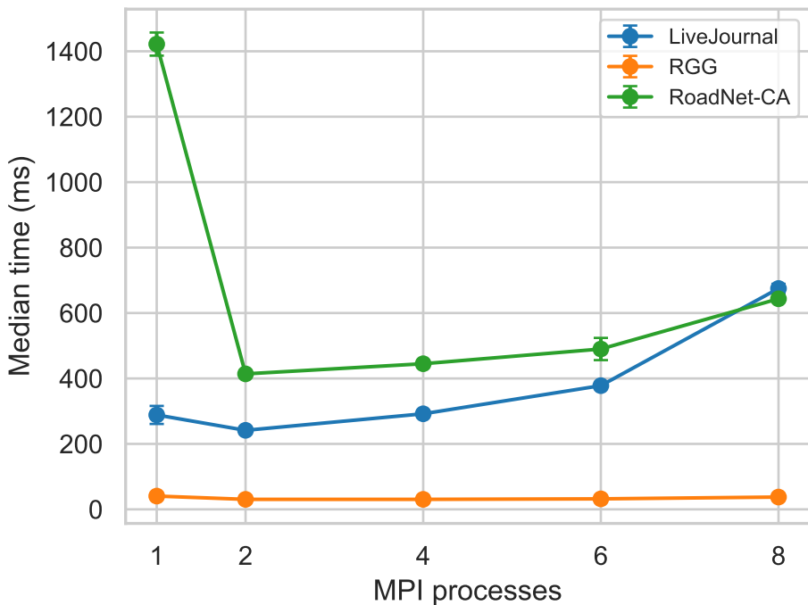
BFS — Execution Time
