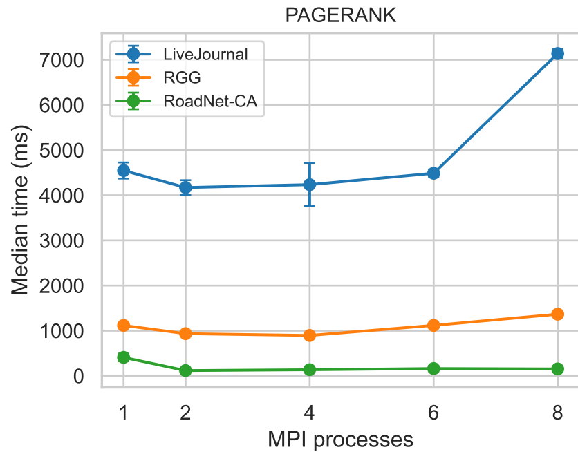
Execution Time vs. Number of MPI Processes
