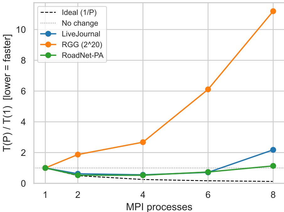
BFS — Normalized Time T(P)/T(1)
