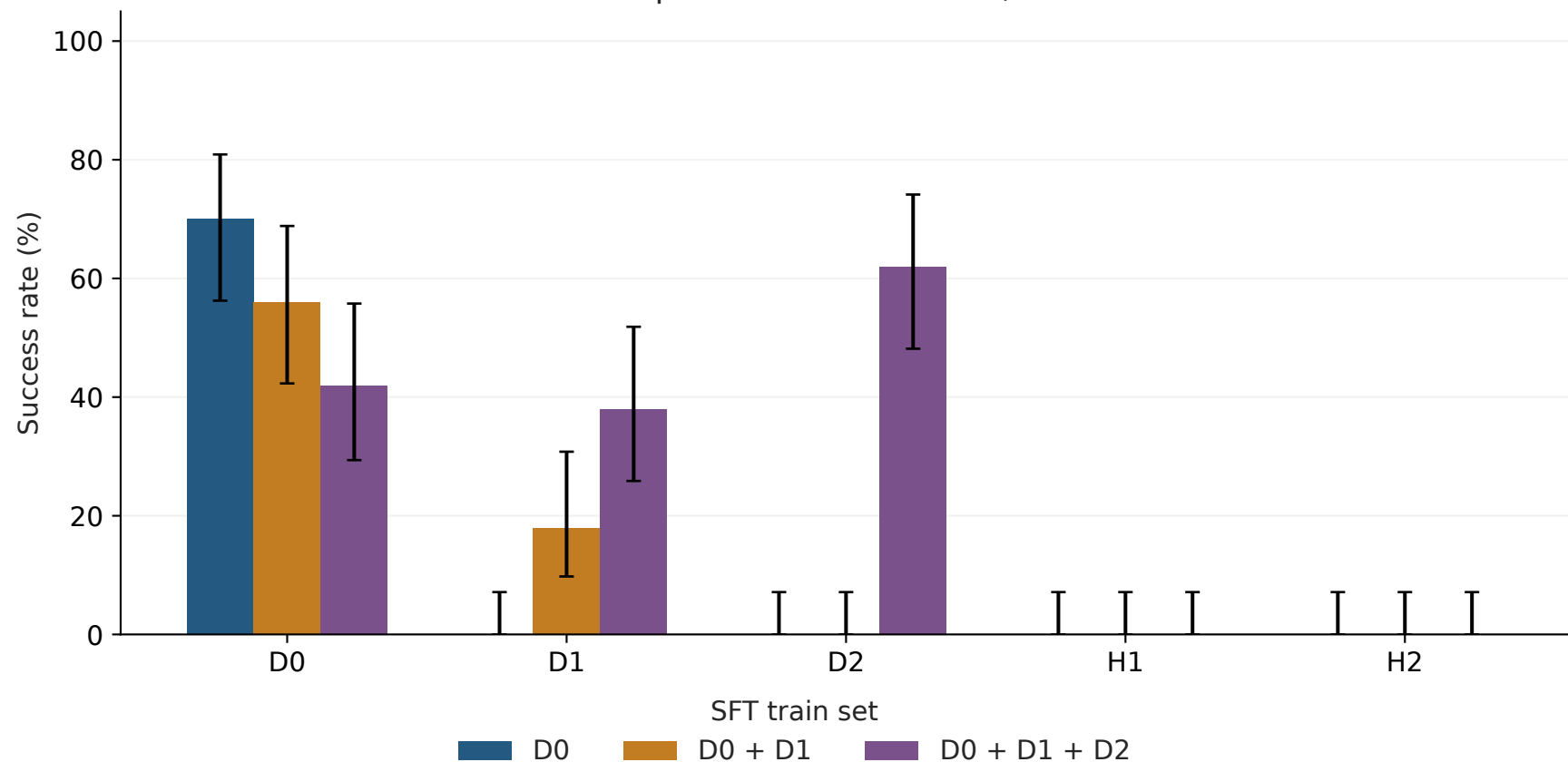
Per-task final performance · N = 50, Wilson 95% CI
