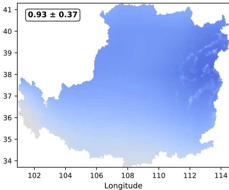
SSP5-8.5 Annual
