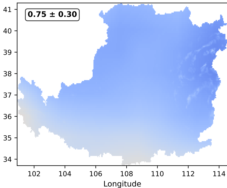
SSP5-8.5 Annual
