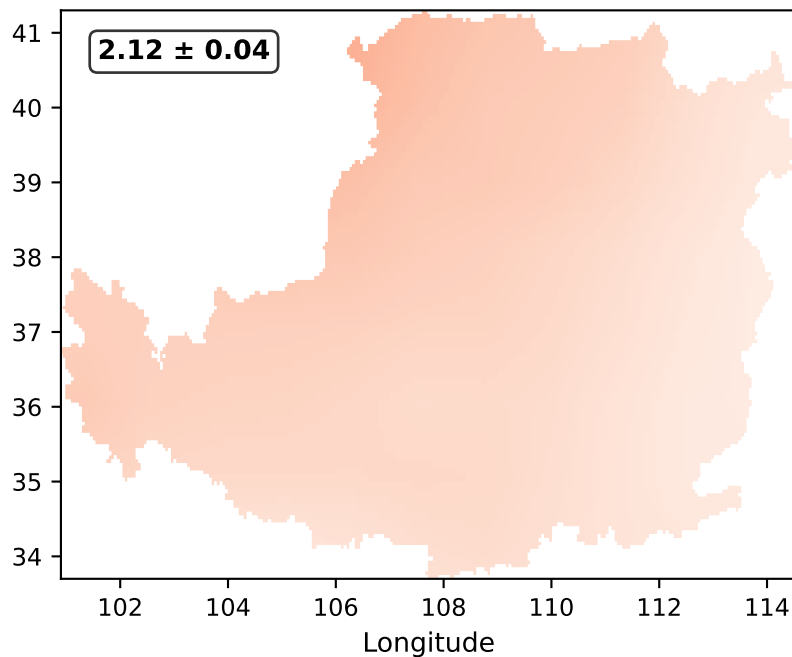
SSP5-8.5 Annual
