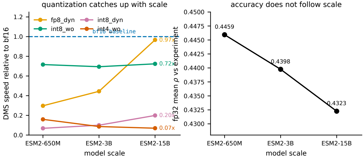
Figure 2: Left : DMS speed relative to bf16 against scale. fp8_dyn converges on bf16 while the weight-only and INT4 paths do not. Right : fp32 mean Spearman falls monotonically across a 23-fold parameter increase. No pairwise difference is significant, but there is no evidence that scale buys variant-effect accuracy, and 15B costs 5.4 \times the compute of 3B for the lowest of the three.
