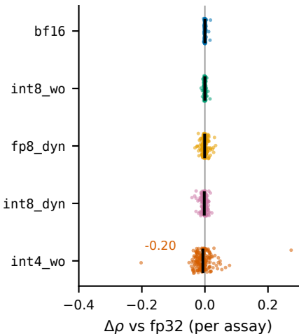
ESM2-650M
