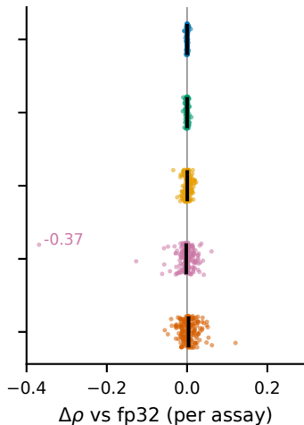
ESM2-3B
