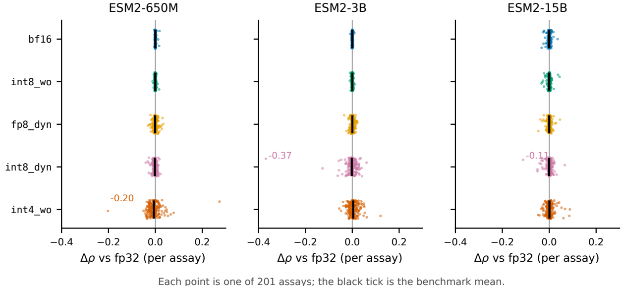
Figure 1: Per-assay change in ground-truth correlation, all 201 assays, all three scales. Black ticks are the benchmark mean, within 0.007 of zero everywhere. bf16 and int8_wo are tight at every assay and scale; int8_dyn and int4_wo have equally unremarkable means and tails reaching -0.37 and -0.20 .
