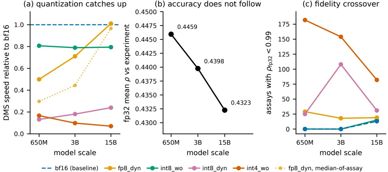
Figure 2: Three effects visible only across scale. (a) DMS speed relative to bf16, as aggregate throughput: fp8_dyn converges on bf16 while the weight-only and INT4 paths do not. The dotted line repeats fp8_dyn under the median-of-assay convention — the only configuration for which the choice is visible, because its overhead is fixed per call and so worst on the short assays a median weights most heavily. (b) fp32 mean Spearman falls monotonically across a 23-fold parameter increase; no pairwise difference is significant, but there is no evidence that scale buys variant-effect accuracy. (c) Number of assays where a configuration drifts from fp32 ( \rho_{fp32} < 0.99 ): bf16 and int8_wo acquire a tail only at 15B while int4_wo sheds one.
