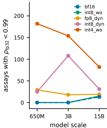
(c) fidelity crossover
