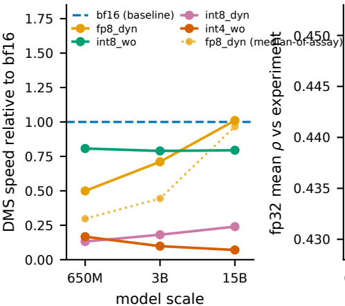
(a) quantization catches up
