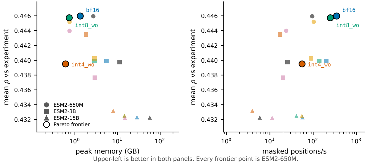
Figure 4: All eighteen scale/configuration combinations on two projections of the Pareto surface; upper-left is better. Circled points are non-dominated and all are ESM2-650M.
