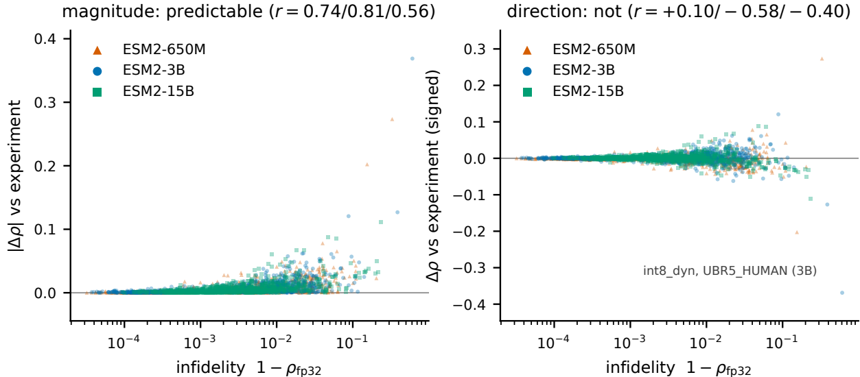
Figure 3: Drift from fp32 against change in ground-truth correlation, 1005 pairs per scale. Left : infidelity bounds the magnitude of the change. Right : signed, the distribution is a symmetric funnel rather than a trend, and the correlation changes sign between scales.
