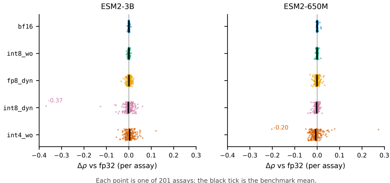
Figure 1: Per-assay change in ground-truth correlation for each configuration, across all 201 ProteinGym assays and both model scales. Black ticks mark the benchmark mean, which is within 0.007 of zero everywhere. bf16 and int8_wo are tight at every assay; int8_dyn and int4_wo have means that are equally unremarkable and tails that reach -0.37 and -0.20 . Selection on the mean cannot distinguish these cases; selection on the tail separates them immediately.
