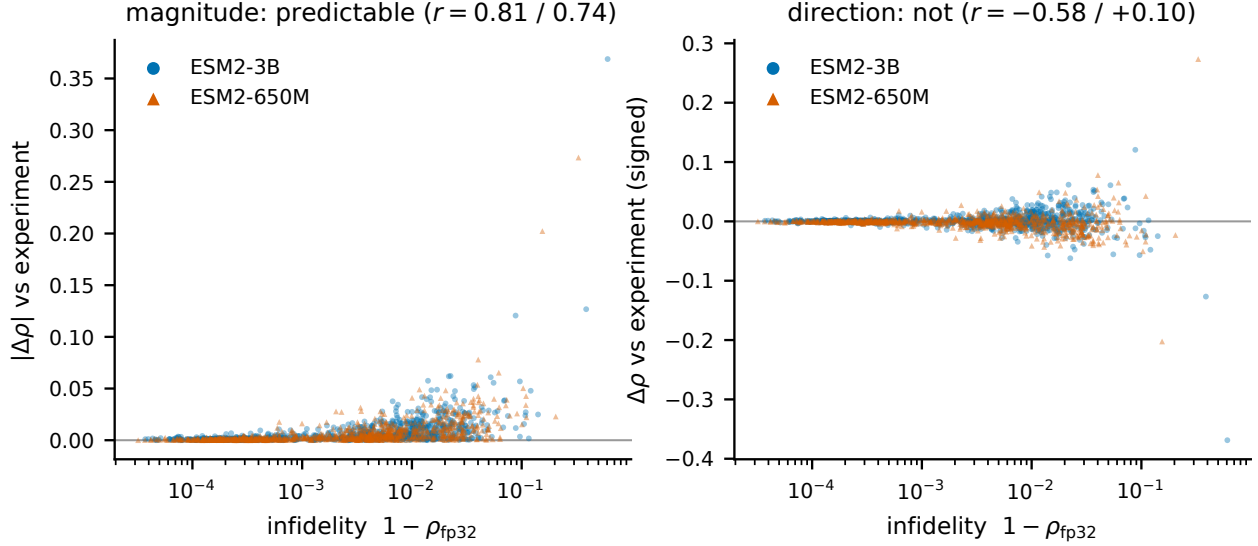
Figure 2: Drift from fp32 against change in ground-truth correlation, over 1005 assay/configuration pairs per model. Left : infidelity bounds the magnitude of the change — the envelope widens monotonically, and nothing far from fp32 is reliably close to it on the ground truth. Right : the same data, signed. The distribution is a symmetric funnel rather than a trend, and the correlation reverses sign between model scales ( -0.58 at 3B, +0.10 at 650M). A small drift is therefore a valid safety certificate, while a large drift is not evidence of a worse model.
