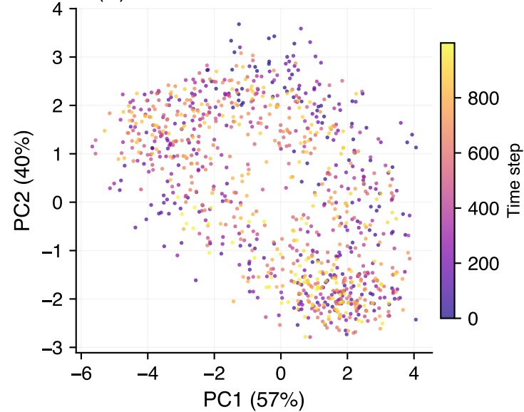
(B) Network state — stimulated
