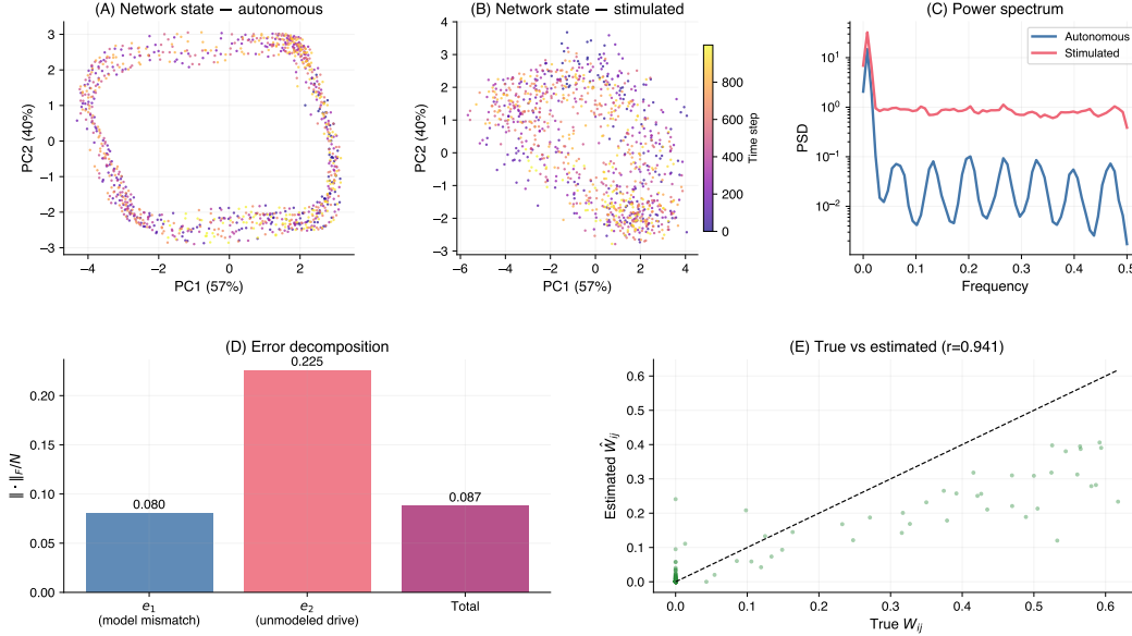
Figure 9: Network dynamics, error decomposition, and recovery quality ( N=15 , \phi = \tanh , \rho(W)=1.0 ). (A–B) PCA phase portraits of network activity ( X \in \mathbb{R}^{T \times N} projected onto PC1–PC2, colored by time via plasma colormap: dark purple \rightarrow yellow). (A) Under autonomous dynamics ( \sigma = 0 ), the trajectory is confined to a low-dimensional manifold shaped by intrinsic oscillators. (B) Under stimulation ( \sigma = 1.0 ), the trajectory fills a larger volume in PC space, reflecting the expanded covariance coverage that enables estimation. (C) Power spectral density (Welch’s method) averaged across neurons. Autonomous dynamics (blue) show concentrated spectral peaks at intrinsic-oscillator frequencies; stimulated dynamics (red) exhibit a flatter spectrum reflecting white-noise input. (D) Error decomposition: \|e_1\|_F/N (model mismatch) vs. \|e_2\|_F/N (unmodeled-drive correlation with state) vs. total estimation error \|\hat{W} - W\|_F/N . e_1 and e_2 are Frobenius norms of the individual error components (Eq. 8); the total can be smaller because these components partially cancel across matrix entries. For this representative topology, e_2 is \sim 2.8\times larger than e_1 (median across topologies: \sim 3\times ), identifying the unmodeled state-dependent drive (here, CPG input) as the dominant error source. (E) Scatter plot of true off-diagonal weights W_{ij} (horizontal) vs. Granger-refined estimates \hat{W}_{ij} (vertical) for this representative topology. Pearson r = 0.94 ; dashed line: y = x . Median raw-estimator correlation across all 10 topologies: r = 0.90 .
